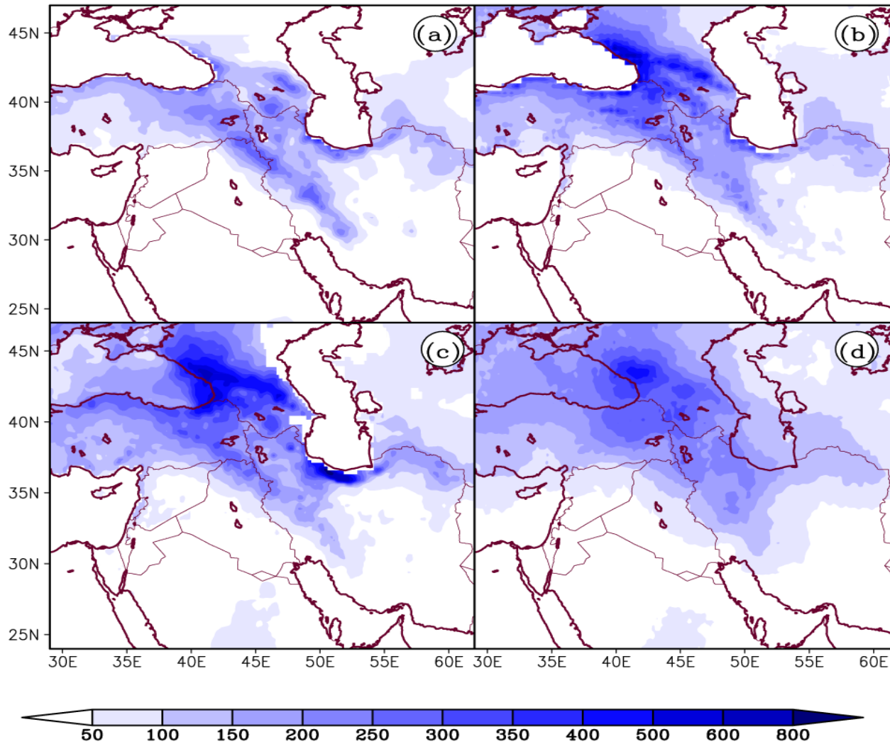
Spatial distribution of 6 month (2004020100 -2004063000) spring total precipitation observation (mm). (a)- AgMMERA (b)-APHRODIT, (c)-CHIRPS & (d)-PERSIAN –CDR.
